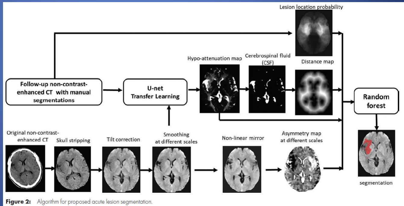
Figure 2: Algorithm for proposed acute lesion segmentation.
