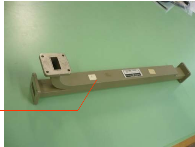
SYSTRON Isolator No. 228
