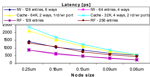
Fig. 1. Latency scaling for Issue Windows (IW), caches and register files (RF). microarchitects assume it as a requirement. The scheduling logic performs two basic operations: Wake-Up and Select . During the Wake-Up phase, instructions in the Issue Window check their dependencies and, if these are resolved, they request access to a functional unit for execution. During the second phase, some of these instructions are selected and scheduled. To be able to schedule dependent instructions in the next clock cycle, the output of a previous Select operation must be available when Wake-Up starts. Thus, these two operations must be executed together during a single cycle.
