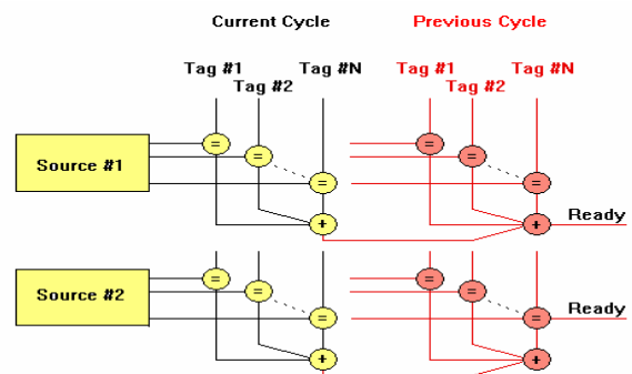
Fig. 5. Duplicated tag matching for the Dual Clock Issue Window.
