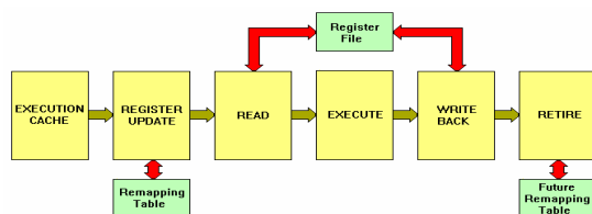
Fig. 10. Equivalent pipeline in trace execution mode
