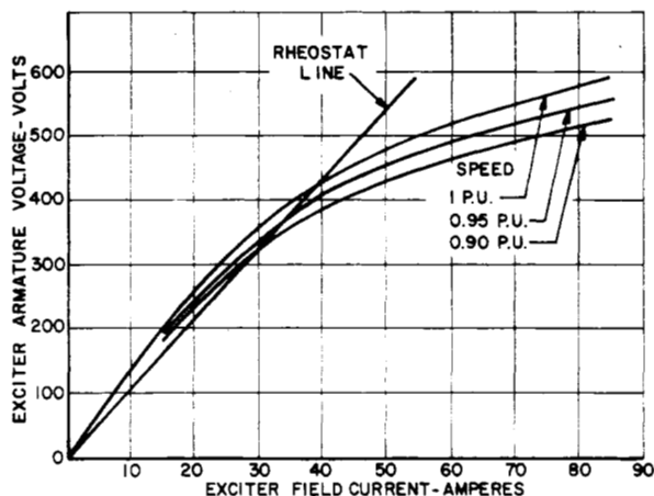
Fig. 11. Typical Saturation Curve for a 500 Volt Shaft Driven Exciter.
