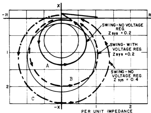
Fig. 9. Loss of Synchronism Characteristics for a Tandem Compound Generator.
