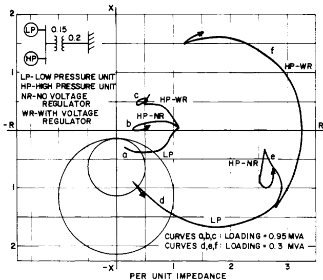
Fig. 4. Loss of Excitation Characteristics for a Cross Compound Generator.
