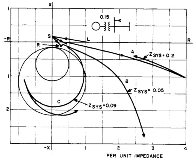
Fig. 8. Stable Transient Swings - Tandem Compound Generator.
