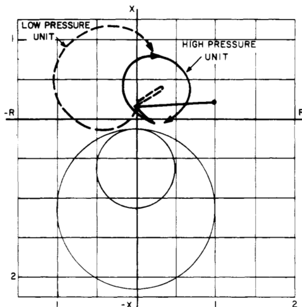
Fig. 10. Loss of Synchronism Characteristics for a Cross Compound Generator.
