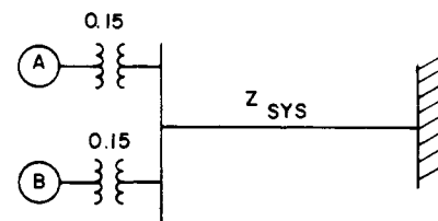
Fig. 6. Two Tandem Compound Generators in Same Station.
