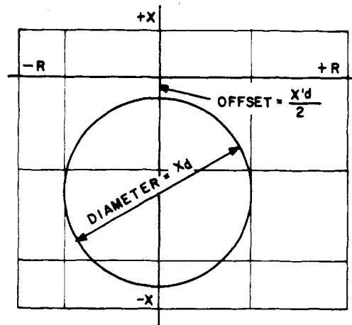
Fig. 1. Operating Characteristic of Loss of Excitation Relay.
