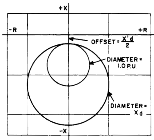
Fig. 13. Generator Protection Using Two Loss of Excitation Relays.
