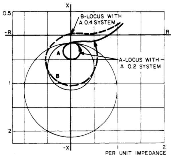
Fig. 12. Impedance Loci During an Underfrequency Disturbance - Tandem Compound Generator.
