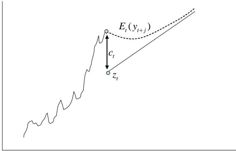
Figure 10.4: Beveridge-Nelson decomposition
