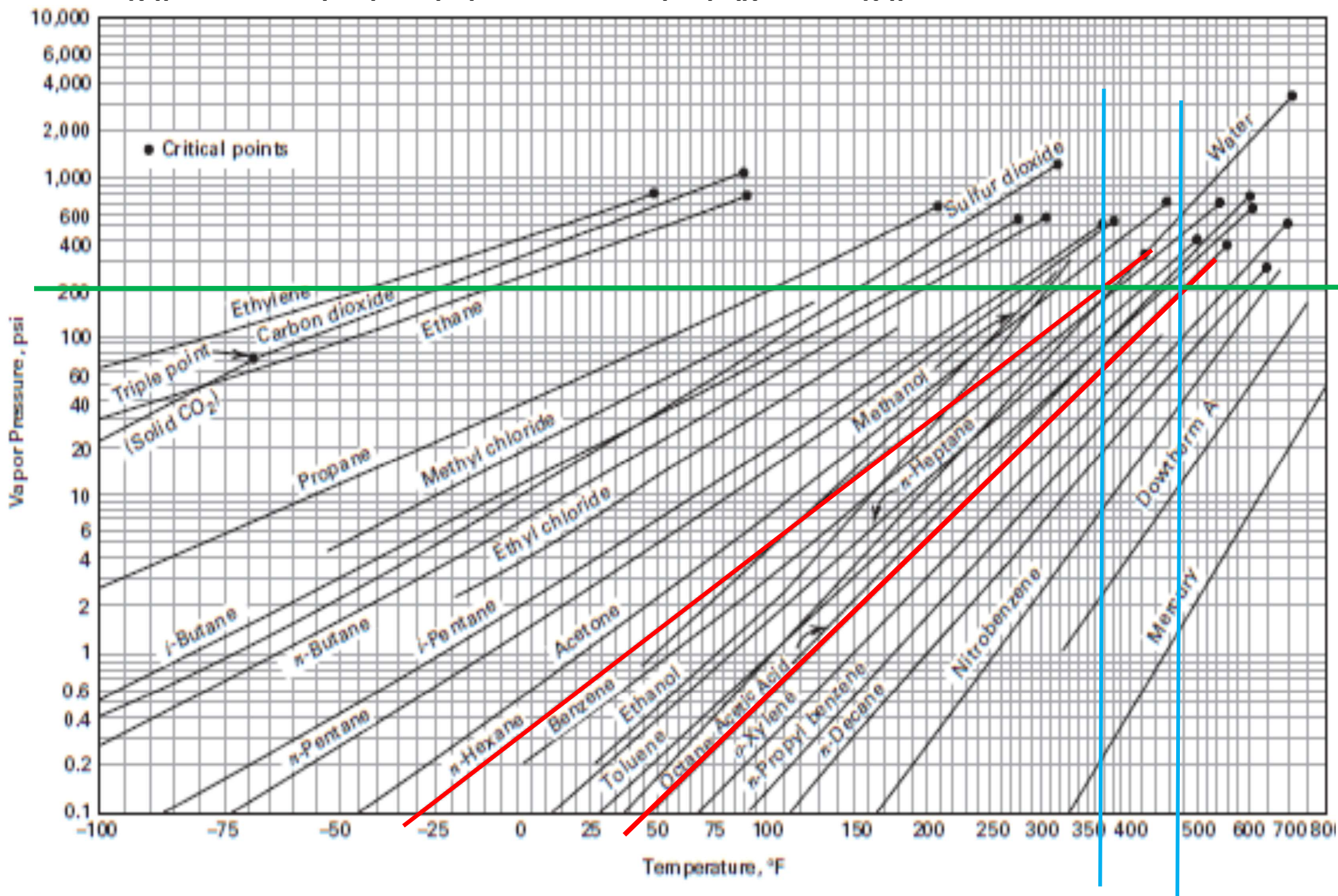
Figure 2.1 Vapor pressure of some common industrial chemicals.
