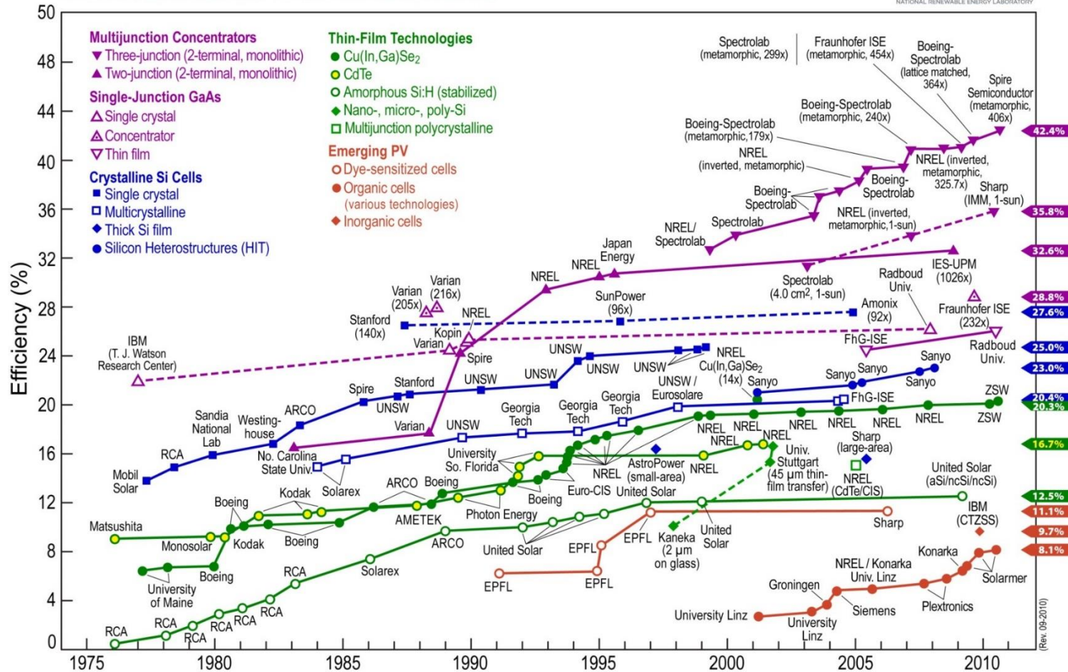
Best Research-Cell Efficiencies
