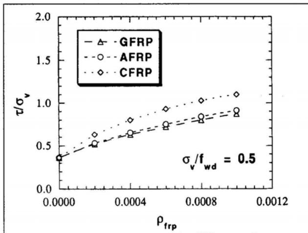
Fig. 6 - Maximum shear stress versus FRP area fraction for a given vertical stress and three types of FRP tendons.
