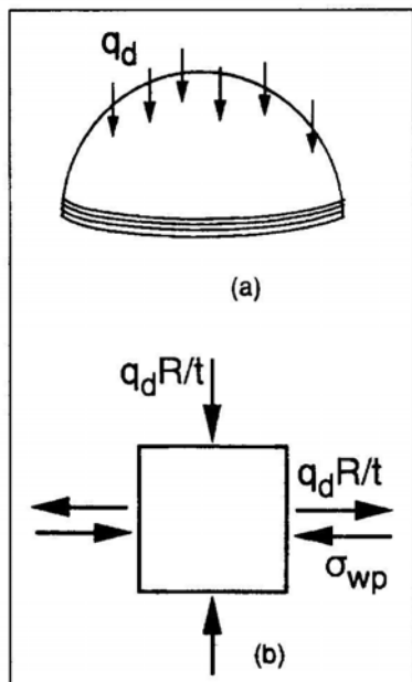
Fig. 7 - (a) Semi-spherical dome under vertical loading; (b) state of stress near the base.
