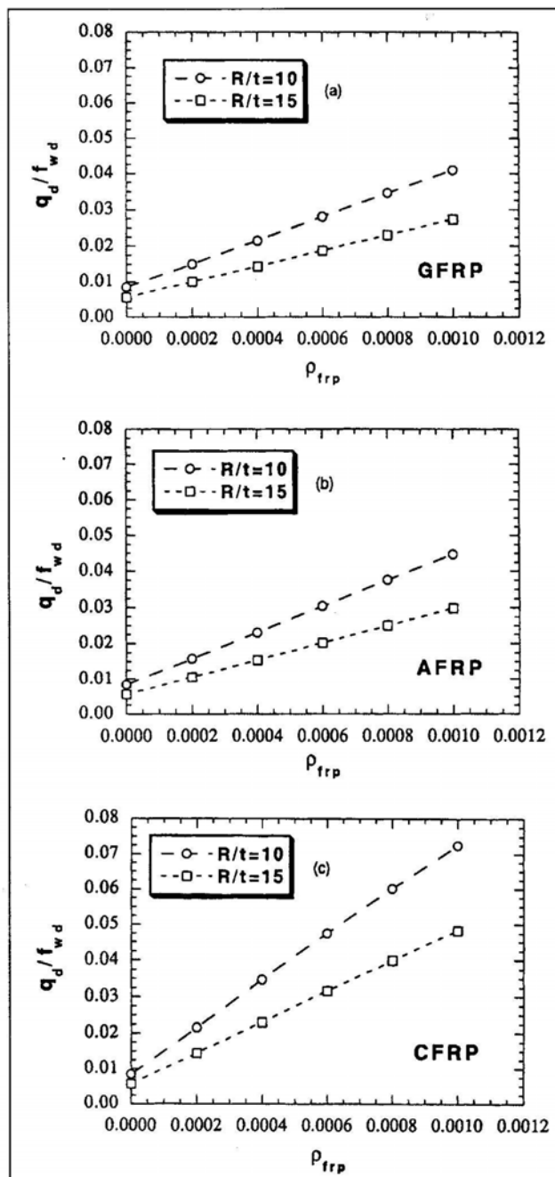
Fig. 8 - Maximum vertical load versus FRP area fraction for two different R/t ratios: (a) GFRP; (b) AFRP; and (c) CFRP.
