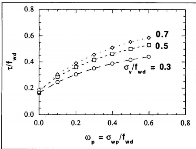
Fig. 4 - Maximum shear stress versus masonry prestress for different vertical stress values.
