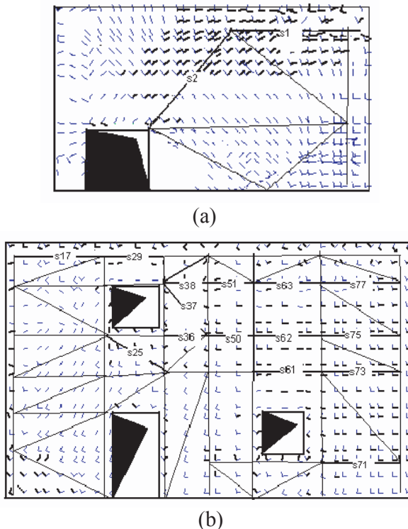
Fig. 4 - Strut-and-tie models.
