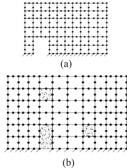
Fig. 2 - Finite element discretization.
