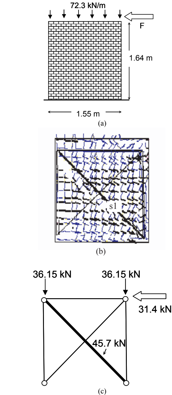
Fig. 6 - (a) Test specimen subjected to in-plane shear. (b) Principal stress fields. (c) Strut-and-tie model, force in the FRP tie at failure.
