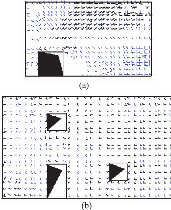
Fig. 3 - Principal stress fields (thick lines represent tension, thin lines compression).
