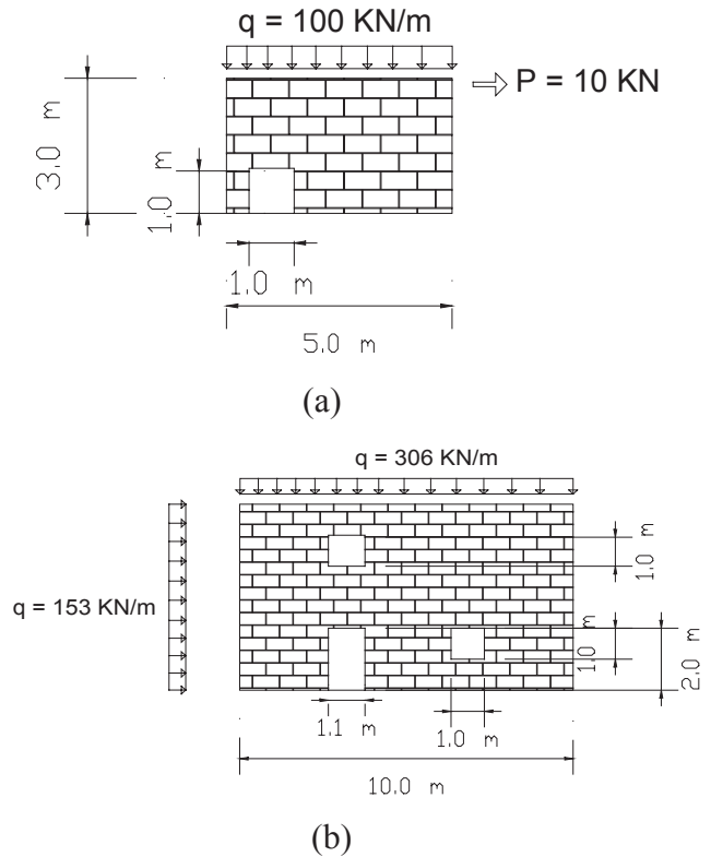
Fig. 1 - Case studies of masonry walls.
