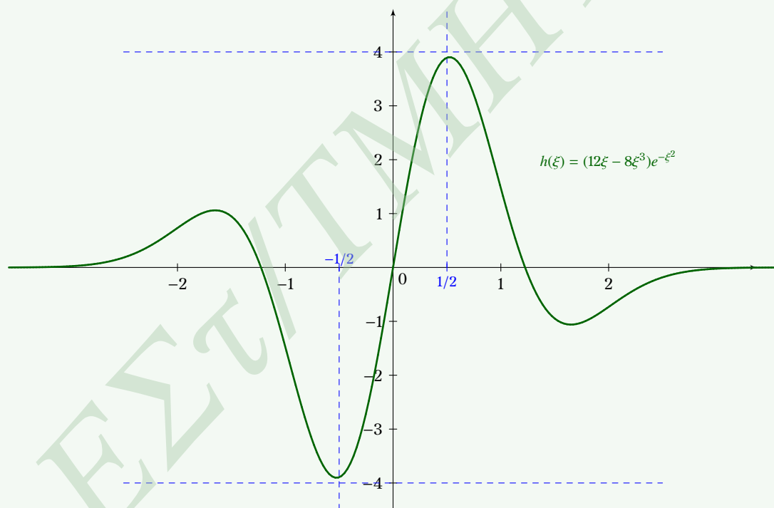
Σχήμα 9.6: R_2(x) = h(\xi)x^2/3!
