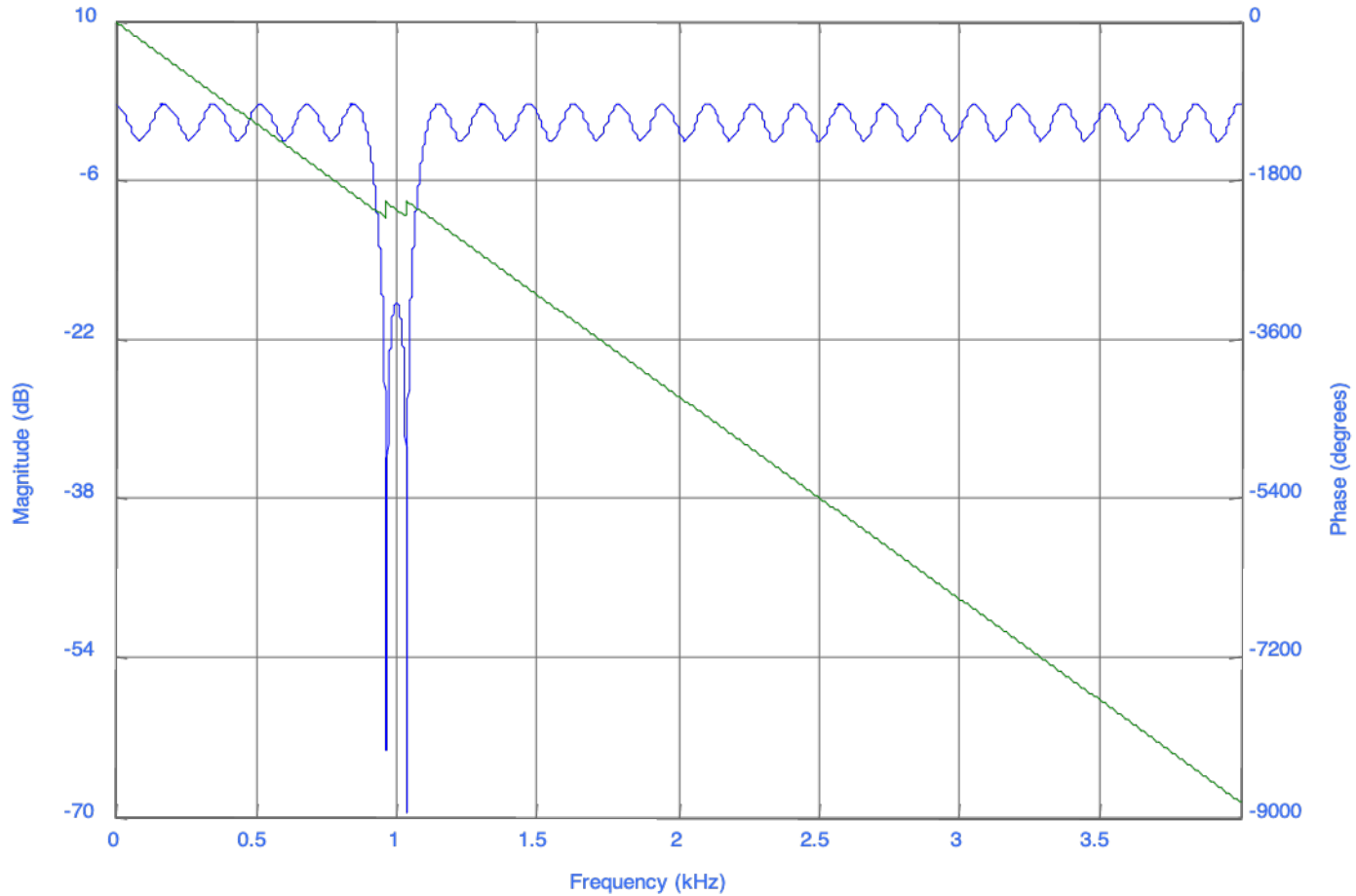
Magnitude (dB) and Phase Responses
