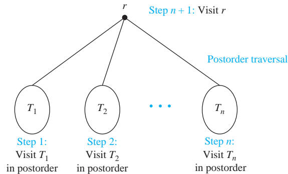
FIGURE 7 Postorder Traversal.
