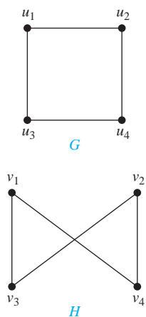
FIGURE 8 The Graphs G and H .
