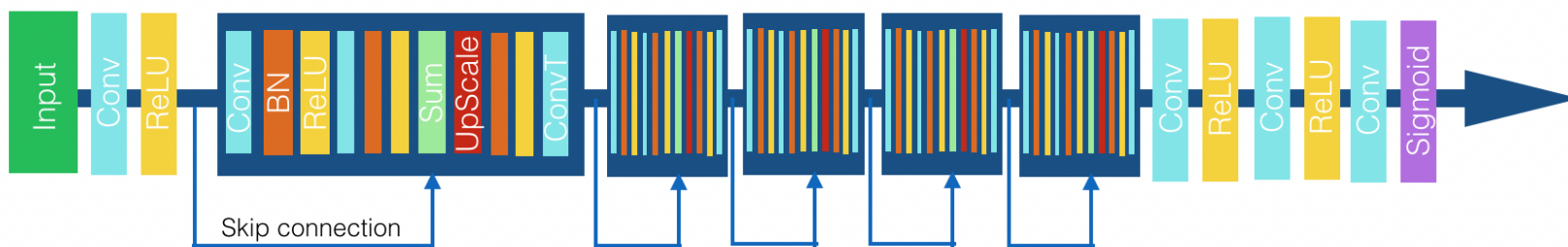
Generator network
