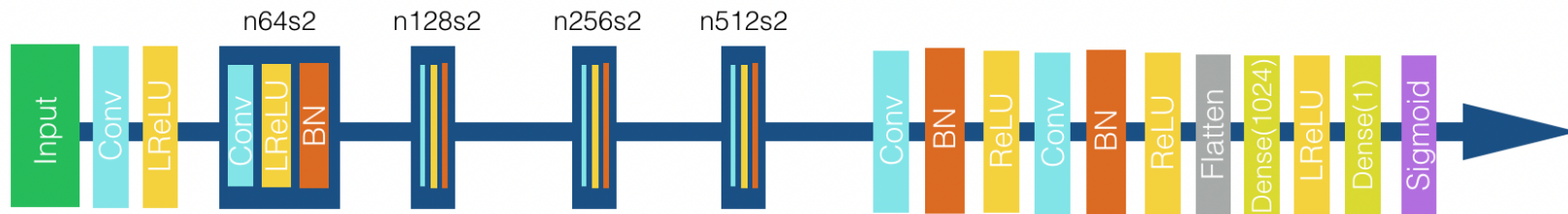
Discriminator network
