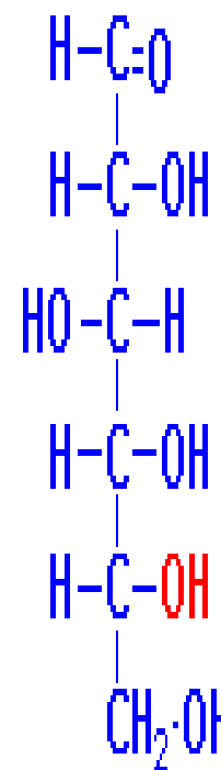
D-glucose
