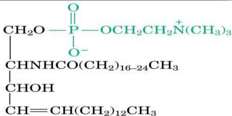
A sphingomyelin
