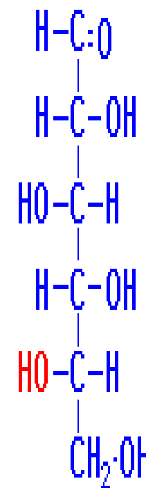
L-glucose
