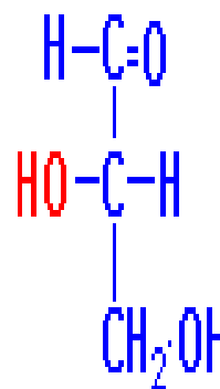
L-glyceraldehyde
