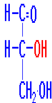
D-glyceraldehyde
