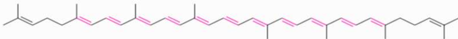
Lycopene, a conjugated polyene
