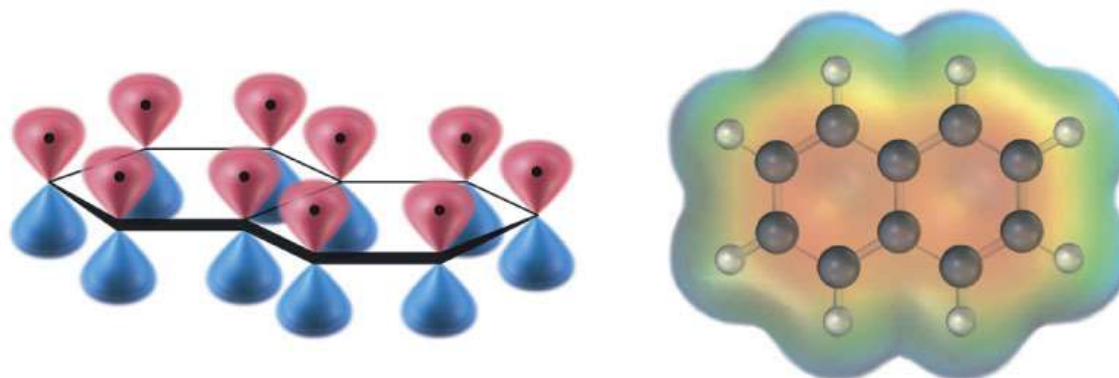
Naphthalene
