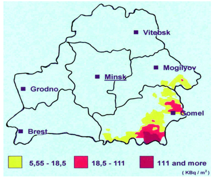
Figure 3-4 Distribution of SR 90
