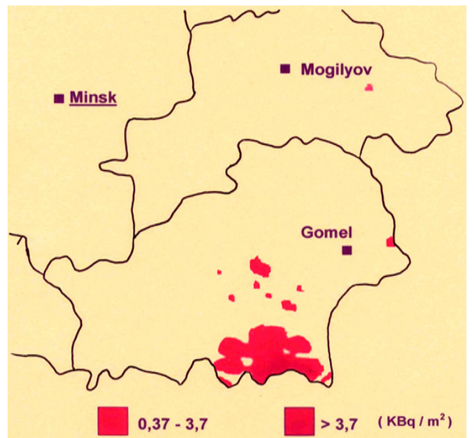
Figure 3-5 Distribution of Pu 238, 239, 240
