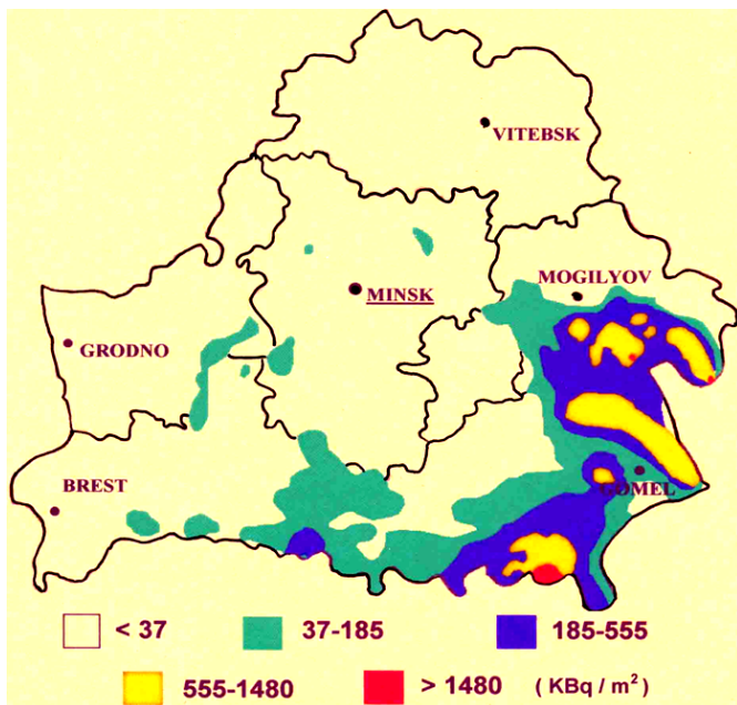
Figure 3-3 Distribution of cesium
