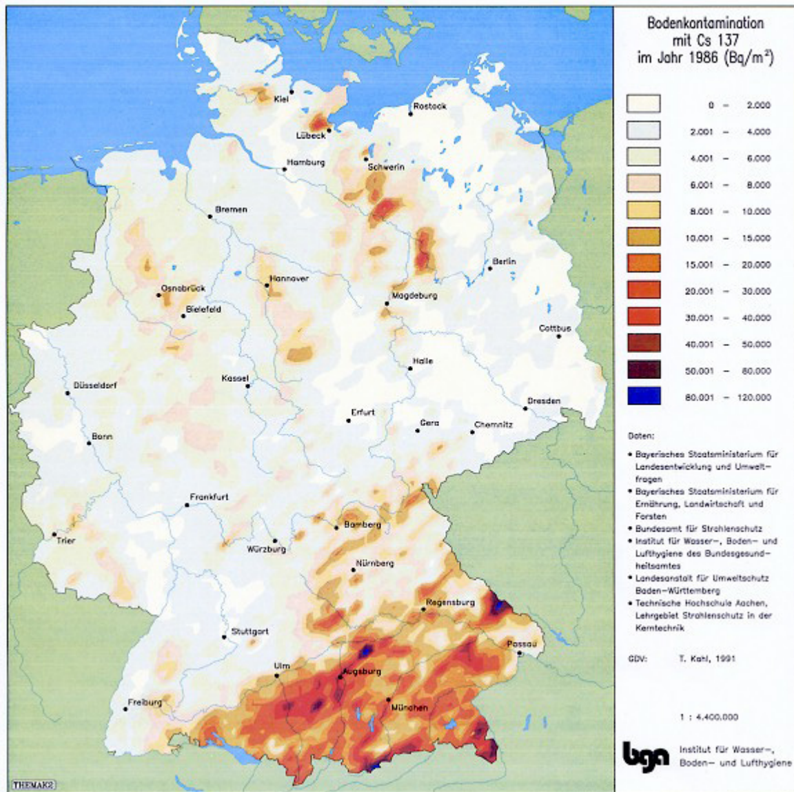
Figure 3-6 Cs 137 soil contamination in Germany
