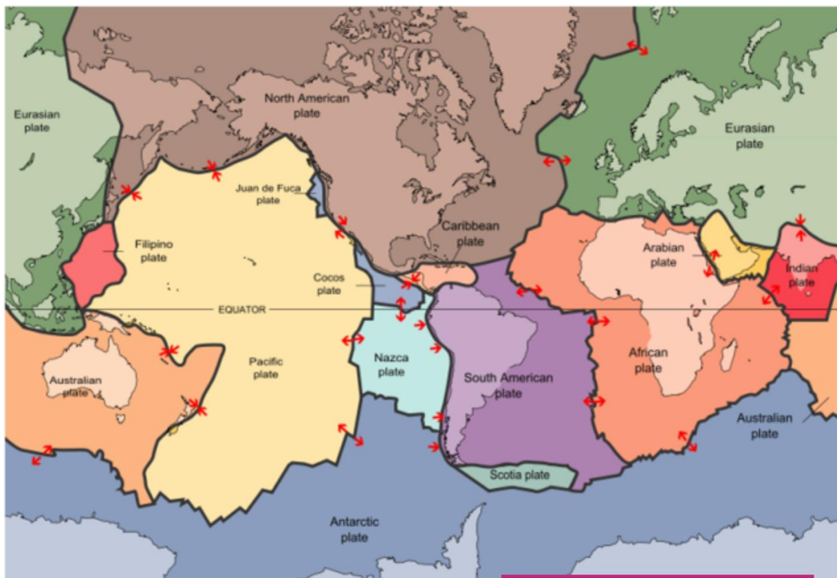
Major and minor tectonic plates
