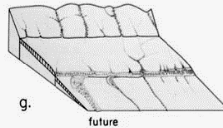
Figure 4. Holocene-late Pleistocene evolution of Wallace Creek. From Sieh and Jahns (1984).
