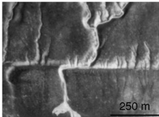
Wallace Creek
