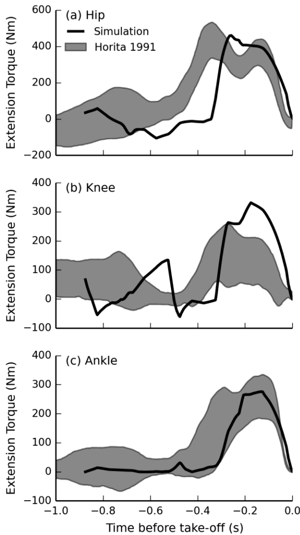
Fig. 4. Joint torques about the (a) hip, (b) knee, and (c) ankle during the ground contact phase for the optimized nominal simulation. The shaded region shows the mean with one standard deviation from experiments. Joint torques from the nominal simulation are shown in the solid line.
