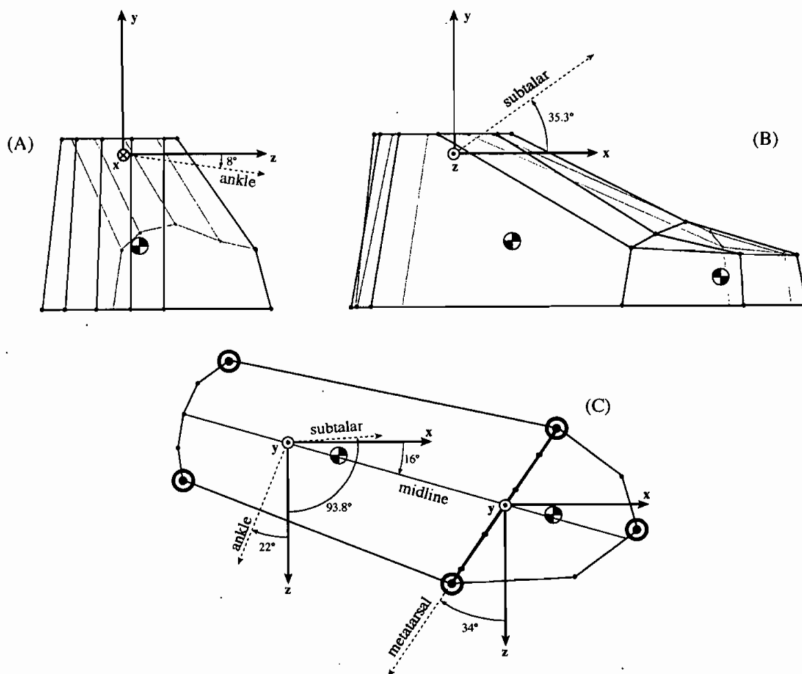
FIGURE 3 Locations of the ankle, subtalar, and metatarsal joint axes for the right foot in the model. The ankle and subtalar axes are projected onto the frontal (A), sagittal (B), and transverse (C) planes. The metatarsal axis is shown in the transverse plane and lies at the sole of the foot (C, metatarsal). The x , y , and z axes define the global reference frame. The vertices and connecting lines represent the volume of a foot plus a size 10 tennis shoe (see text). When the model is in its reference position, the midline of the foot is oriented 16^\circ clockwise from the global x axis (C). Projected onto the transverse plane, the ankle axis is 22^\circ clockwise and the subtalar axis is 93.8^\circ counterclockwise from the global z axis (C). The metatarsal axis is 34^\circ clockwise from the global z axis in the transverse plane (C). Projected onto the frontal plane, the ankle axis is 8^\circ clockwise from the global z axis (A). In the sagittal plane, the subtalar axis is 35.3^\circ counterclockwise from the global x axis (B). The circled dots define the locations of the five ground springs placed under each foot (C).
