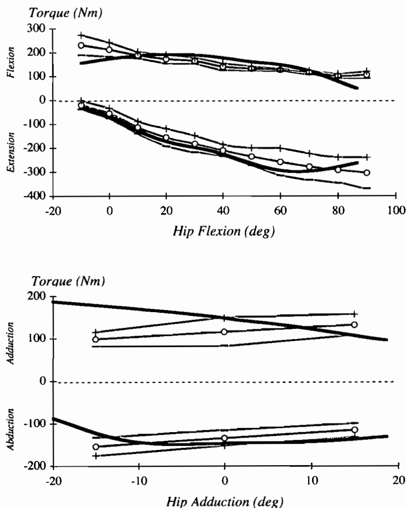
FIGURE A2 Maximum isometric torques generated at the hip in the sagittal plane (flexion-extension) and frontal plane (adduction-abduction) for the model (black lines). The grey lines define the range of maximum torques measured for the five subjects: empty circles are the mean values; + and - indicate 1 SD.
