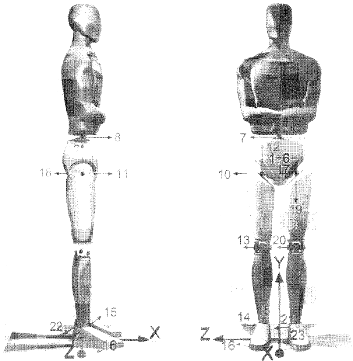
FIGURE 2. Diagram showing the 10-segment, 23 dof model of the skeleton. The numbers indicate the generalized coordinates ( q_i 's). The pelvis is the base segment in the model: generalized coordinates q_1-q_3 specify the position of the origin of the pelvis reference frame with respect to the origin of the inertial reference frame fixed on the ground ( X, Y, Z ); and q_4-q_6 specify the orientation of the pelvis reference frame with respect to the inertial reference frame. On the left side of the body, where appropriate, the axis directions are reversed so that positive changes in the generalized coordinates produce the same anatomical motion. Generalized coordinate q_9 (axial rotation of the HAT) is inside the HAT segment and is not labelled in the figure. See Table II for details.
