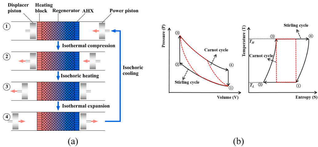
Fig. 1. (a) Operating principle of an SE and (b) P - V and T - S diagrams for ideal Stirling and Carnot cycles.
