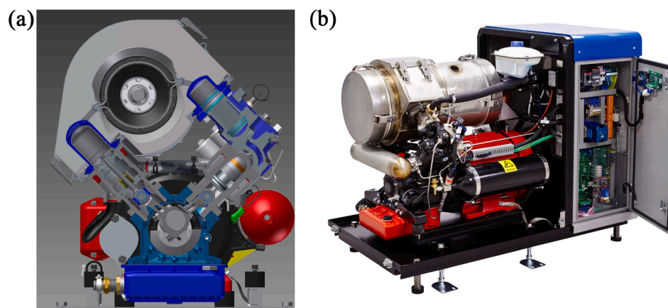
Fig. 13. (a) Section view and (b) photograph of SOLO V161 CHP-unit [91,92].
