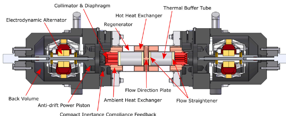
Fig. 5. Cross-sectional view of dual TASEG [27].
