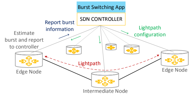
Fig. 13. Optical SDN-based QoS-aware burst switching application [345]: Based on short-term traffic burst estimates of an edge node, the SDN controller configures end-to-end light paths ensuring QoS.
