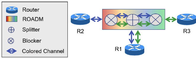
Fig. 7. Broadcast and Select colorful ROADM. The add/drop node, R1, has ports for two optical channels. These channels are directed at the ROADM. The ROADM uses a splitter to broadcast the channels onto two outbound ports, where a wavelength blocker selects the appropriate channel for the next router.
