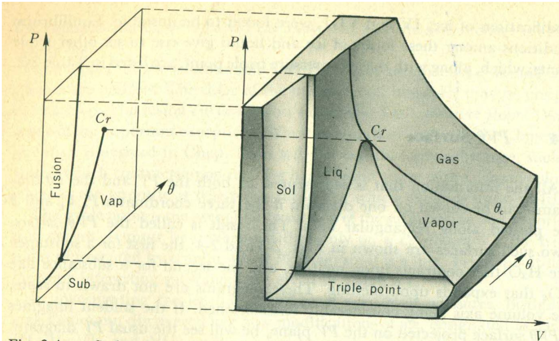
Fig. 2-4 Surface for a substance that expands on melting.
