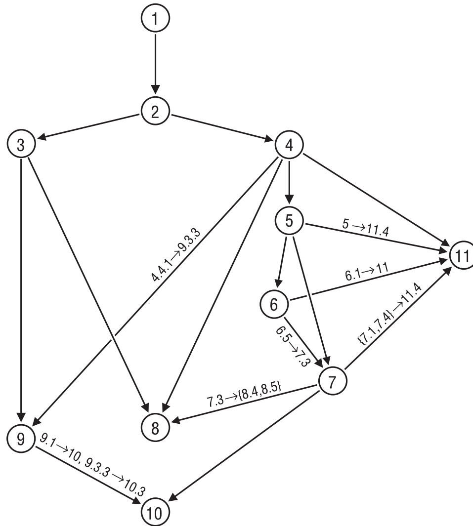
Figure 1.1 Dependency diagram
