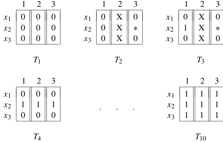
Figure 6.1 An example for n = 3 and t = 1
