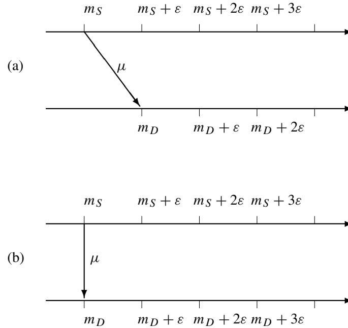
Figure 11.1 The two basic scenarios
