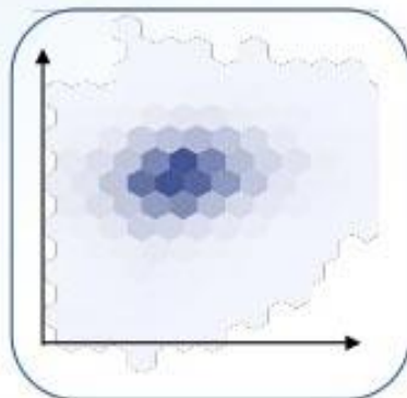
Hexagonal Bin Plot
