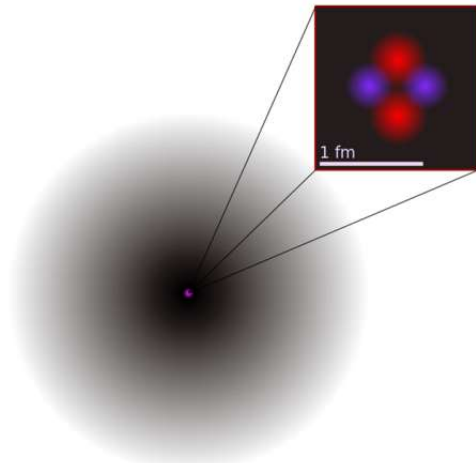
Neutron
