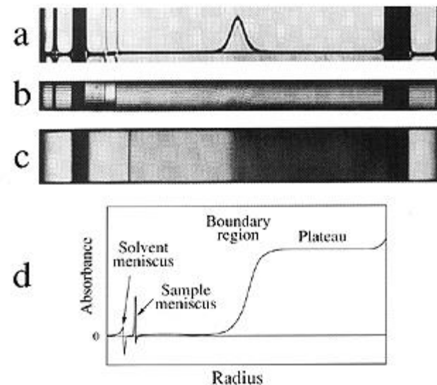
Comparison of the data obtained from the (a) schlieren, (b) interference, (c) photographic absorbance, and (d) photoelectric absorbance optical systems. ((a) (b) and (c) are taken from Schachman, 1959. Reprinted with the permission of Academic Press.)
