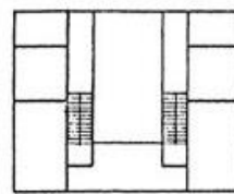
Villa Sarego at Miega
